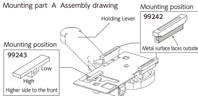
Mounting part A Assembly drawing
