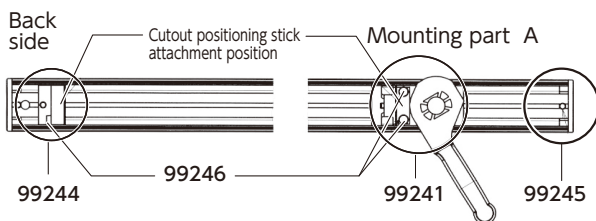
Mounting part A Assembly drawing
